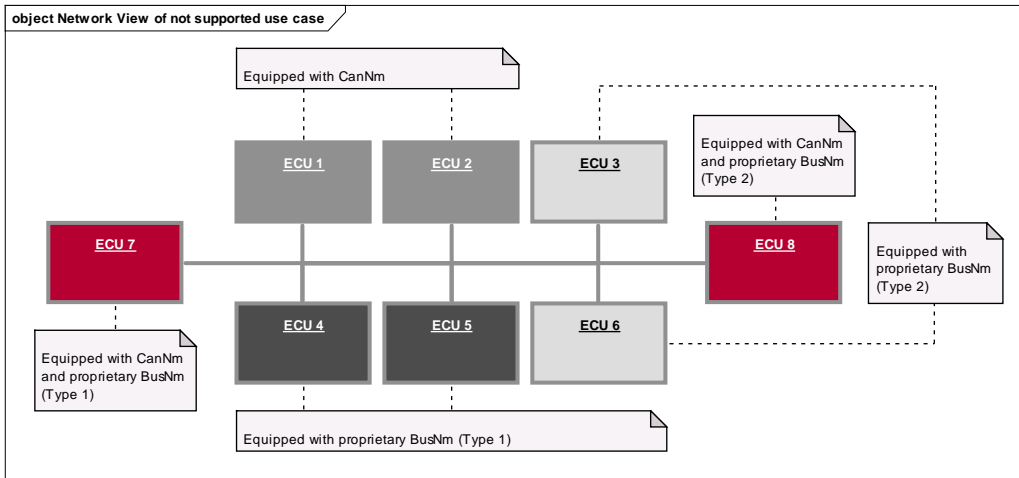
Figure 3-4 Unsupported use case having more than one node with multiple BusNms
