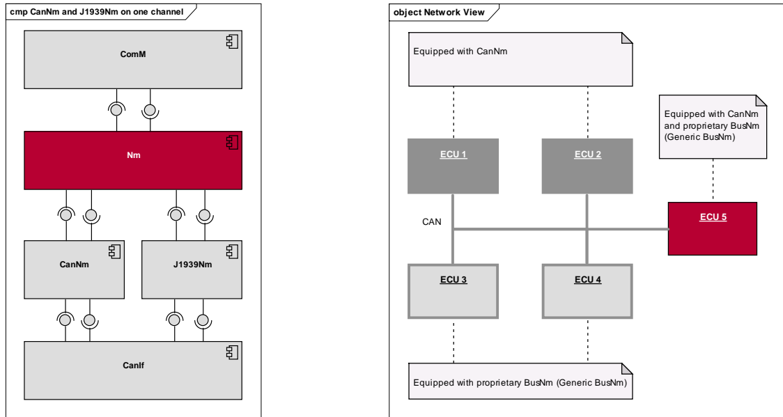
Figure 3-2 Left: Architectural View in AUTOSAR. Right: Network Topology with multiple BusNms on one network
