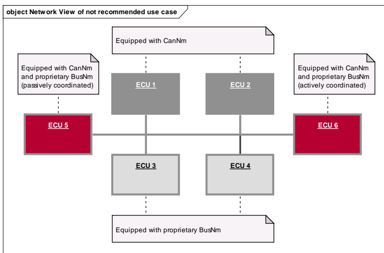
Figure 3-3 Not recommended use case having more than one node with multiple BusNms on the network
