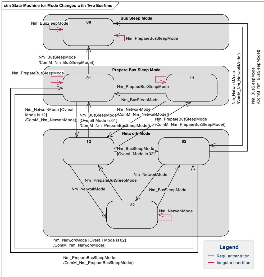
Figure 3-5 Mode Changes with two BusNms on one channel
