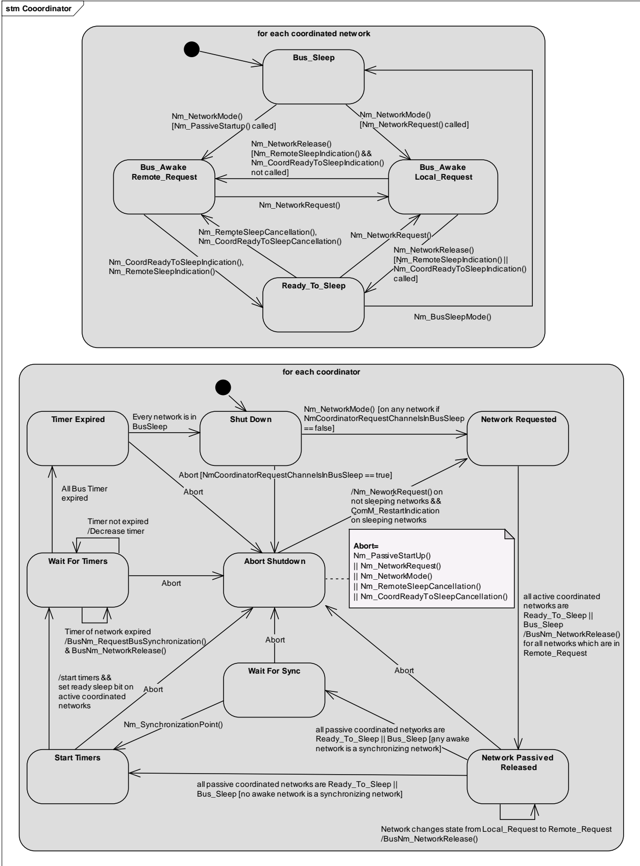
Figure 3-1 State Machine of Coordinator
