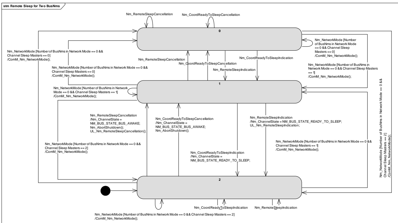
Figure 3-6 State Machine of Remote Sleep callbacks for two BusNMs on one channel
