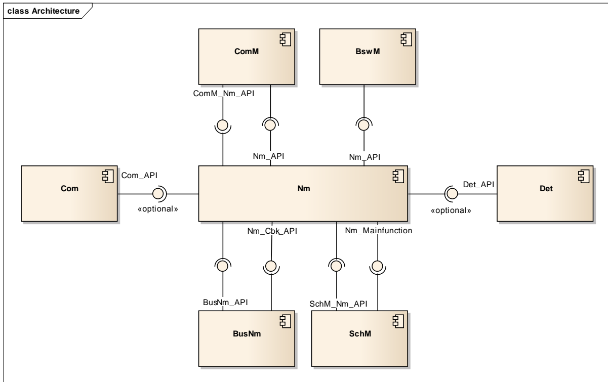
Figure 2-2 Interfaces to adjacent modules of the Nm
