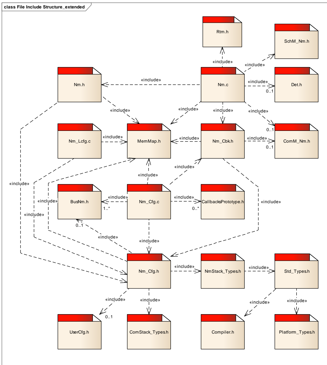
Figure 4-1 Include structure
