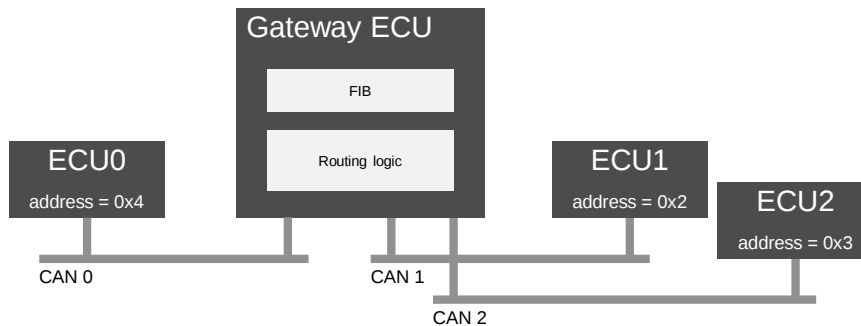
Figure 3-4 Example switching network topology
