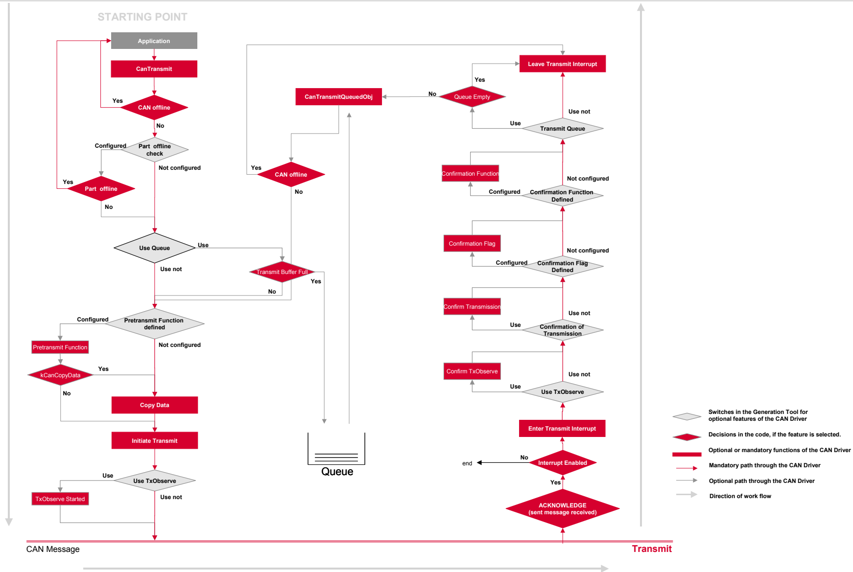
Figure 5-1 Transmission of a CAN message
