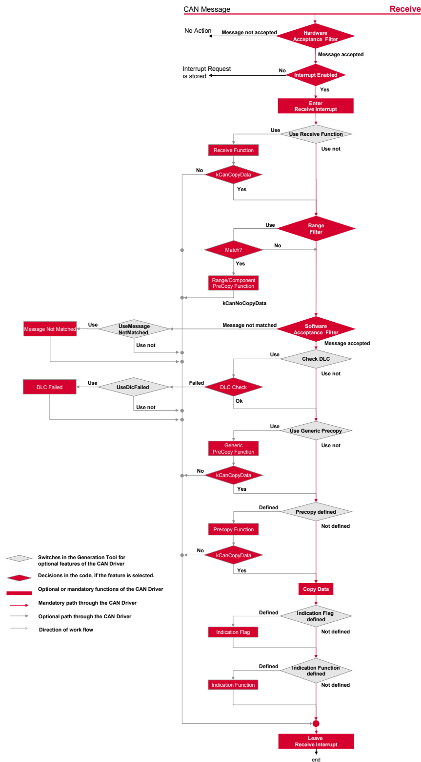
Figure 5-10 Reception of a CAN messages
