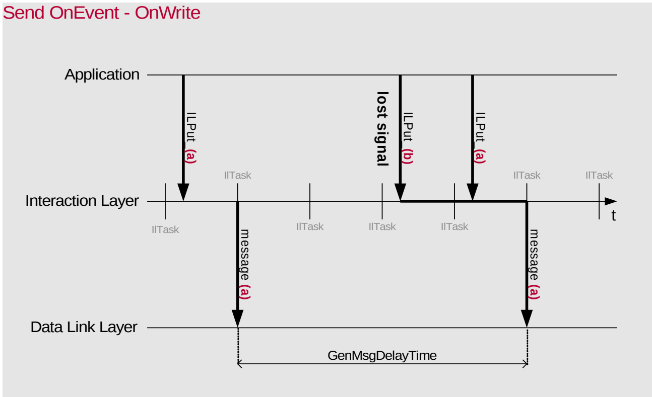
Figure 3-6 Timing Diagram of the Transmission Mode OnEvent – OnWrite
