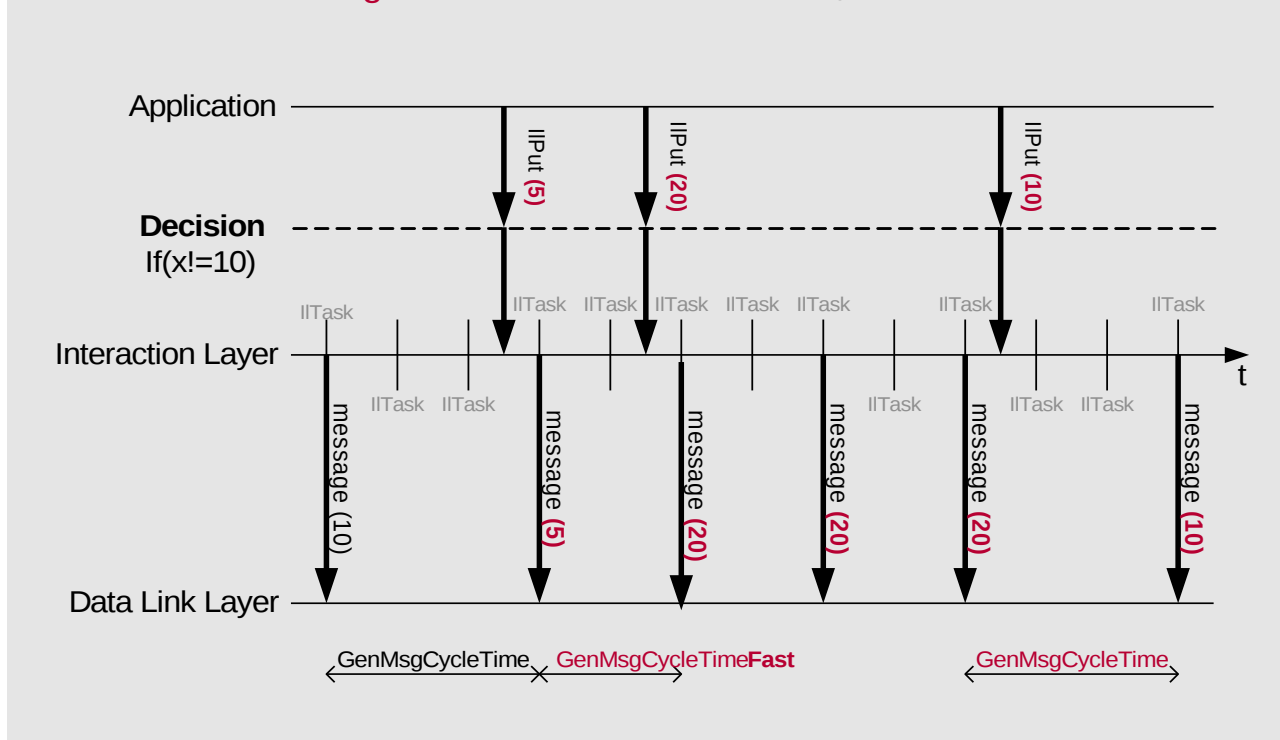
Figure 3-13 Mixed Transmission Mode – Cyclic OR Fast If Signal is Active
