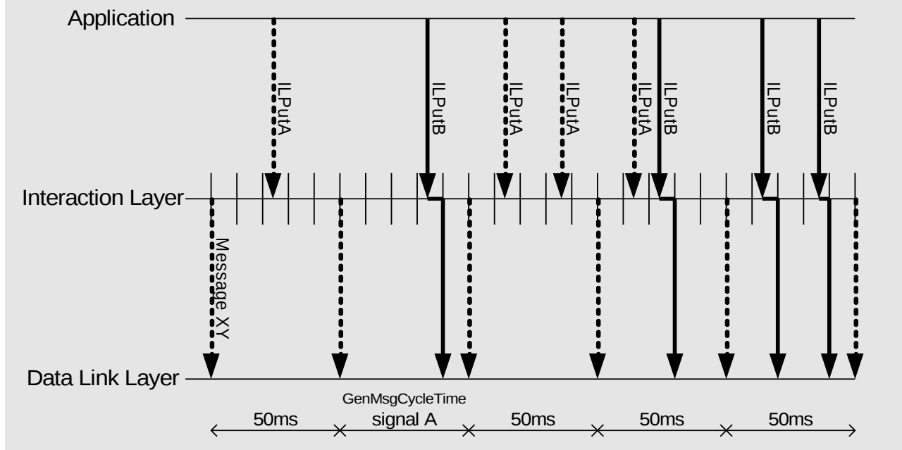
Figure 5-1 A Signal with the Periodic Transmission Mode and one with the Direct Transmission Mode Combined to a message.
