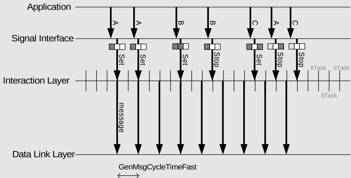
Figure 3-9 Example for Combining Signals Related of the Send Fast if Signal Active Mode to the Same Message
