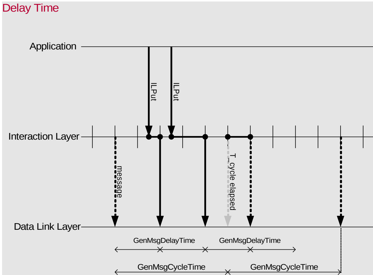
Figure 3-15 Delay Time to Delimit Bus Load
