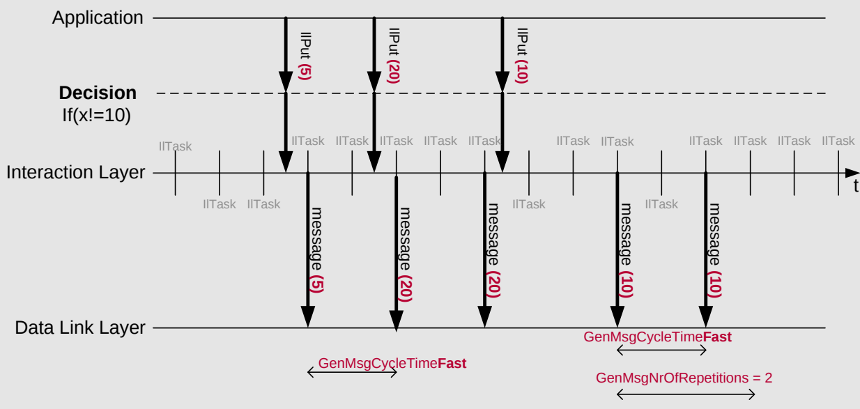
Figure 3-10 Timing Diagram of the Transmit Fast if Signal Active Transmission Mode
