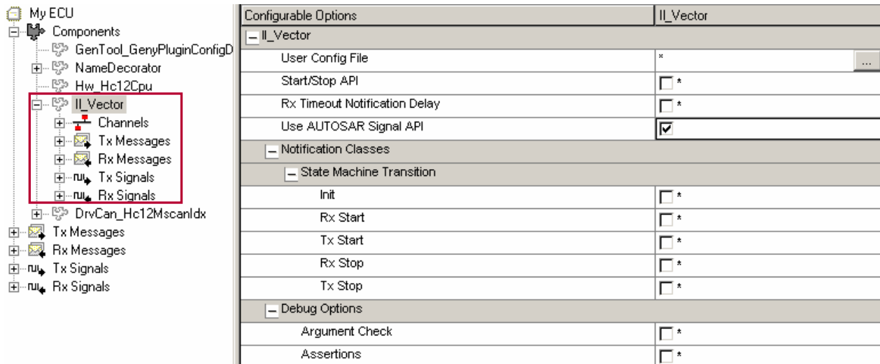
Figure 5-3 Overview of Vector Interaction Layer Configuration in GENy
