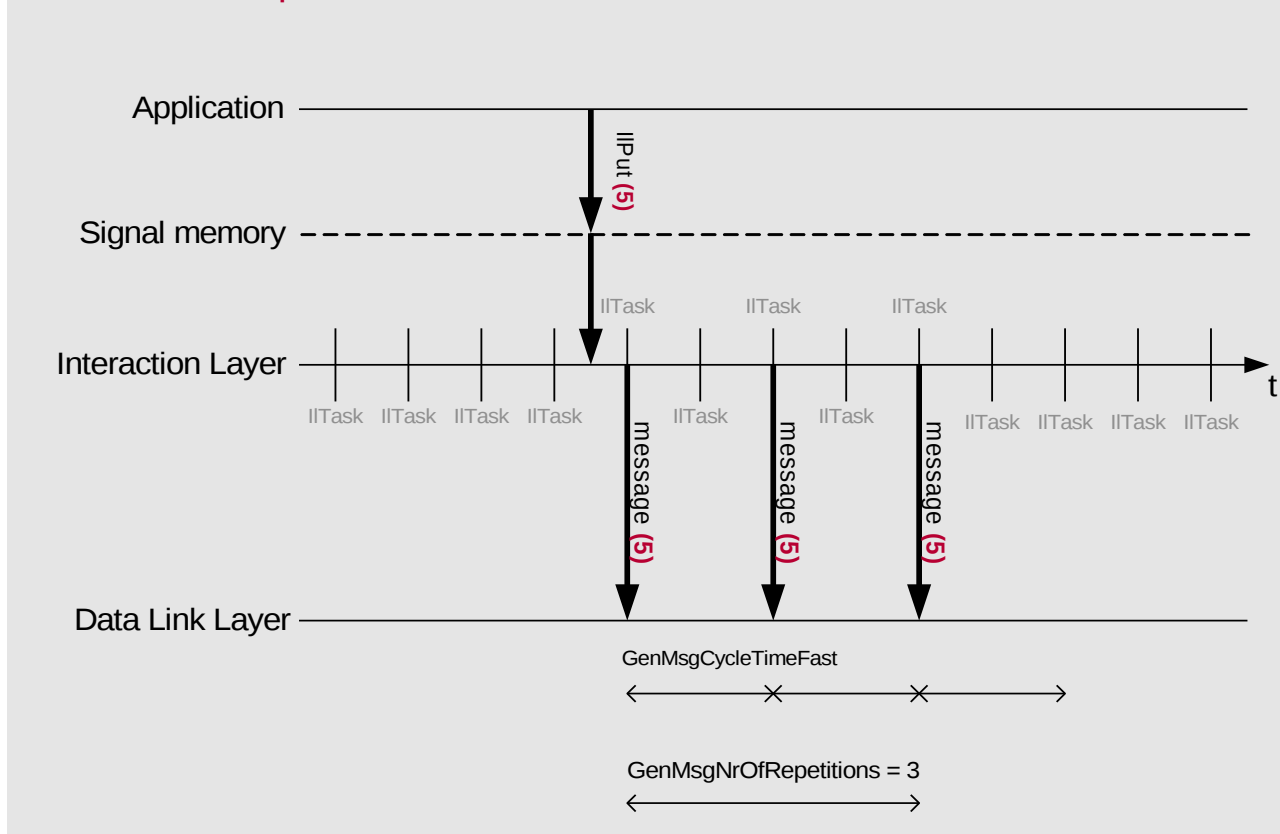
Figure 3-7 Timing Diagram of OnEvent with Repetition - OnWrite
