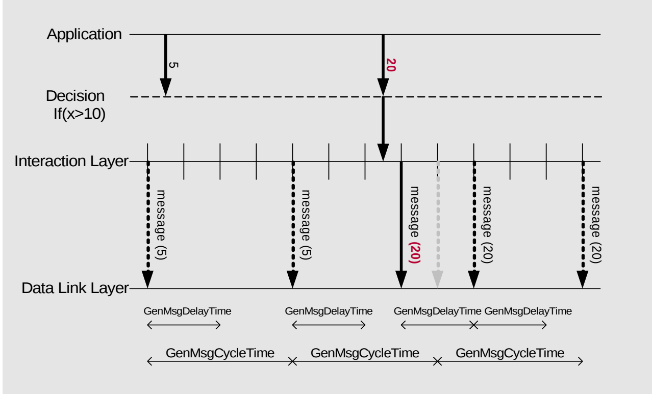
Figure 3-12 Mixed Transmission Mode – Cyclic OR OnEvent [Change]
